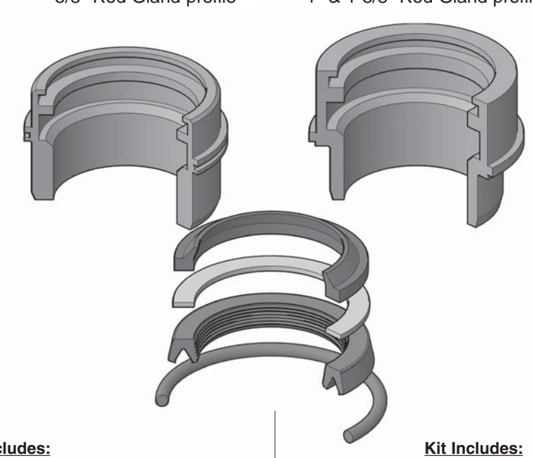
5/8" Rod Gland profile
